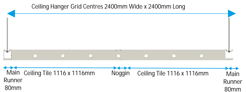
Section View
