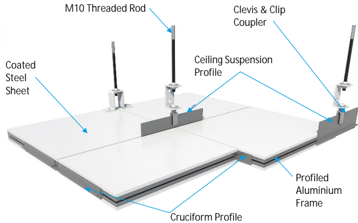
3D View
