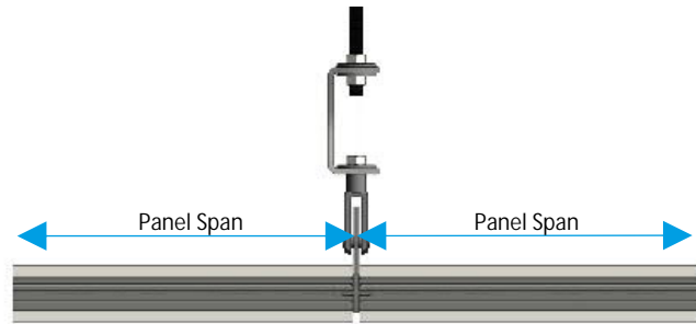
Section View
